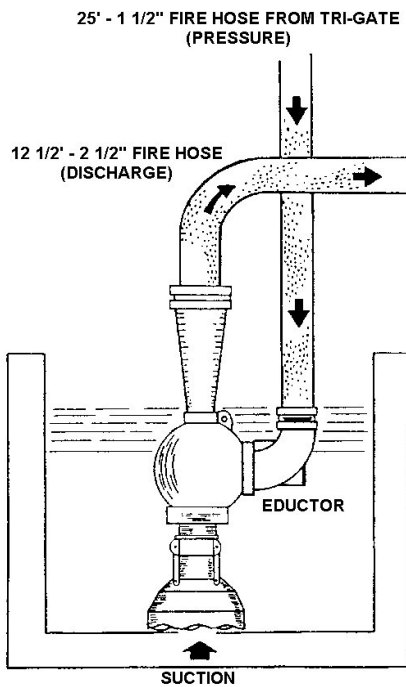
Figure 5-4 Eductor Rigged for Dewatering
