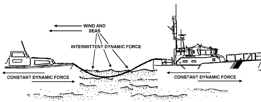
Figure 3-2 Dynamic Forces
