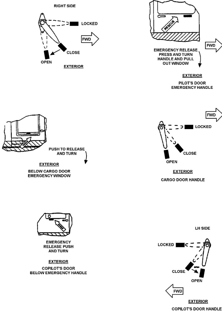
Figure 6-16 MH-60 Emergency Entrances
