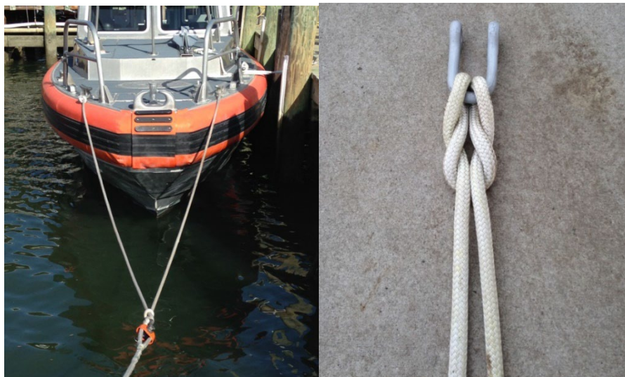
Figure 3-4 Bridle/Cats Paw
