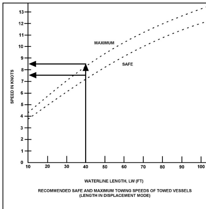
Figure 3-16 Calculated Safe Towing Speeds
