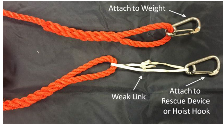
Figure 6-7 Trail Line's Weak Link
