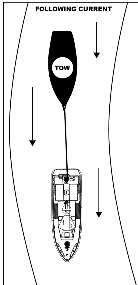
Figure 3-18 Tail Current
