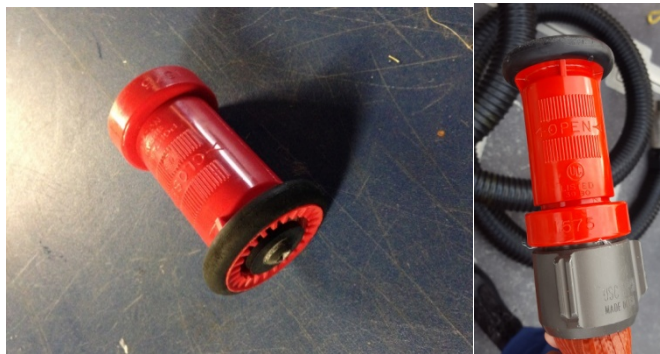
Figure 5-16 Fire Fighting Nozzle
