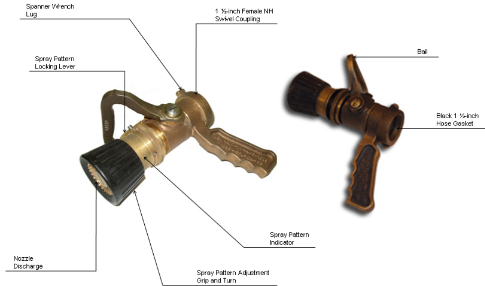
Figure 5-14 Vari-Nozzle
