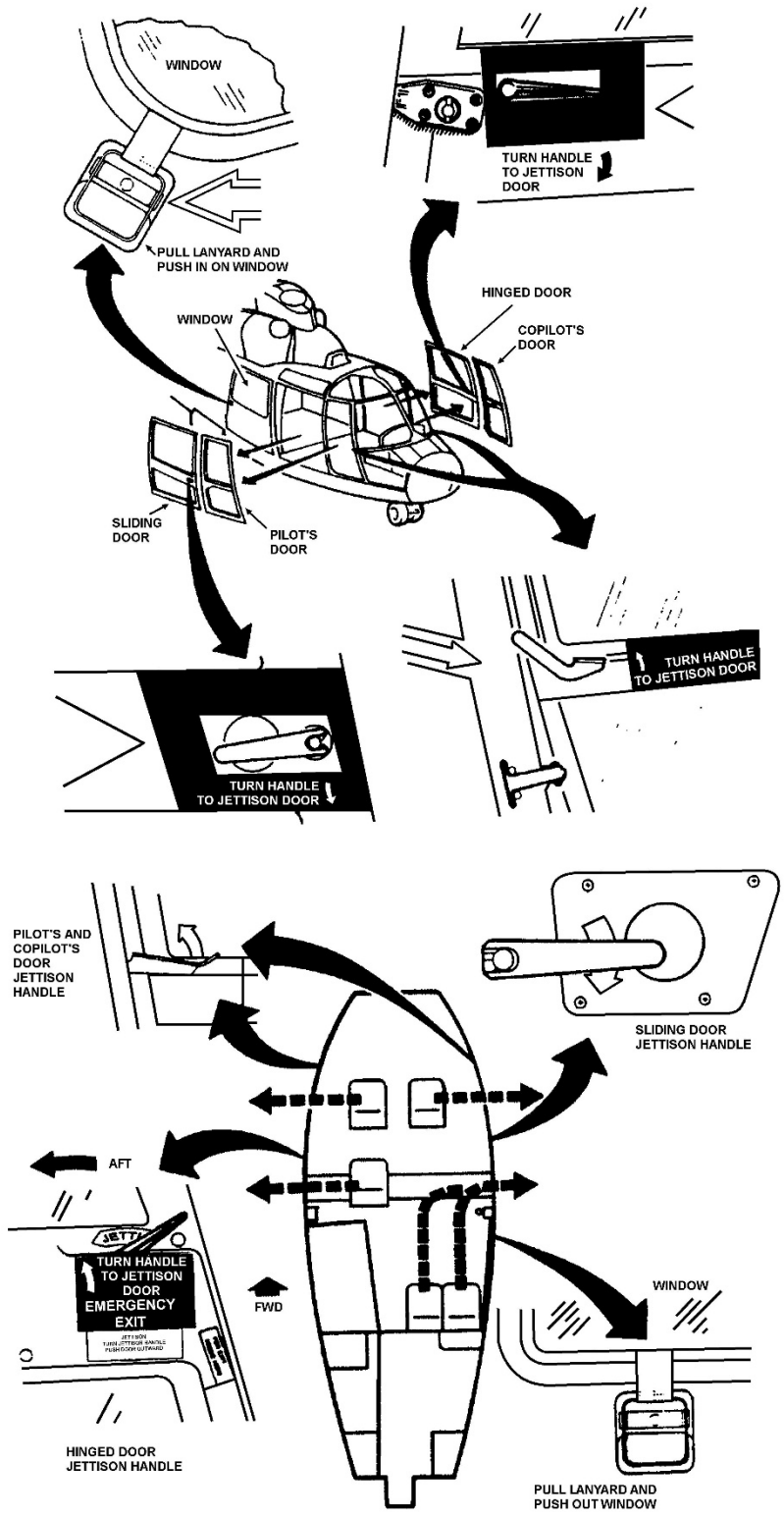
Figure 6-17 MH-65 Emergency Entrances
