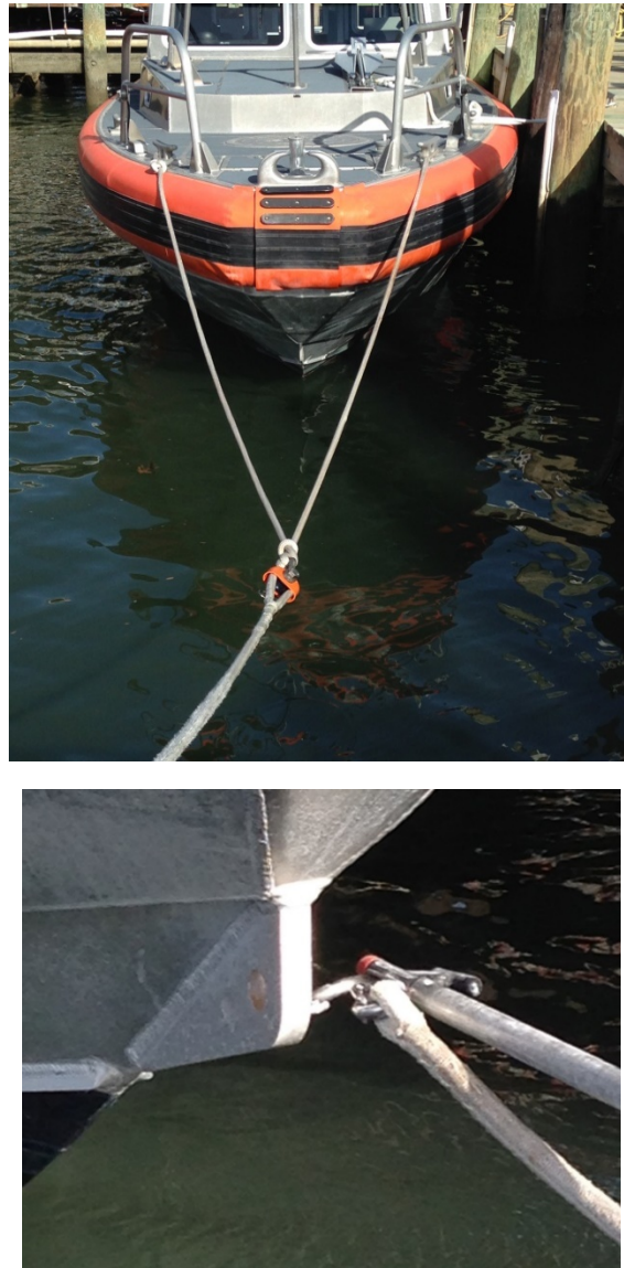
Figure 3-13 Bridle and Trailer Eyebolt Tow Rig Connection
