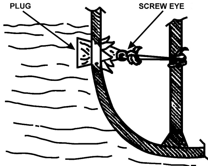
Figure 5-1 Screw Eye
