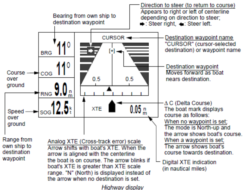
Figure 3-81 GPS Highway Display
