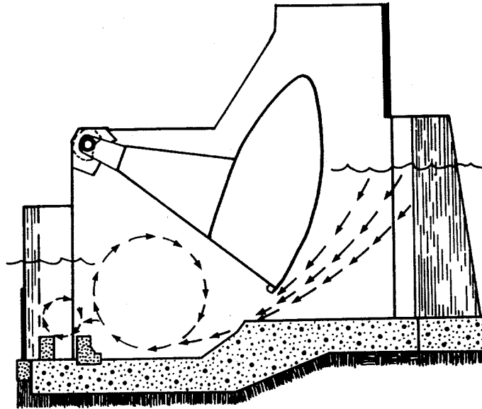
Figure 3-90 Roller Gate Dam
