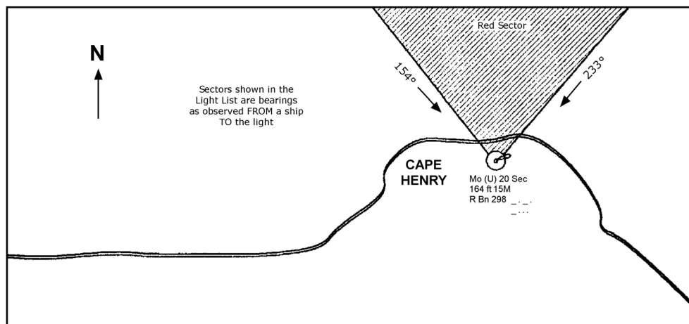
Figure 2-7 Sector Light
