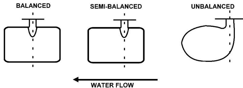
Figure 3-7 Rudder Types
