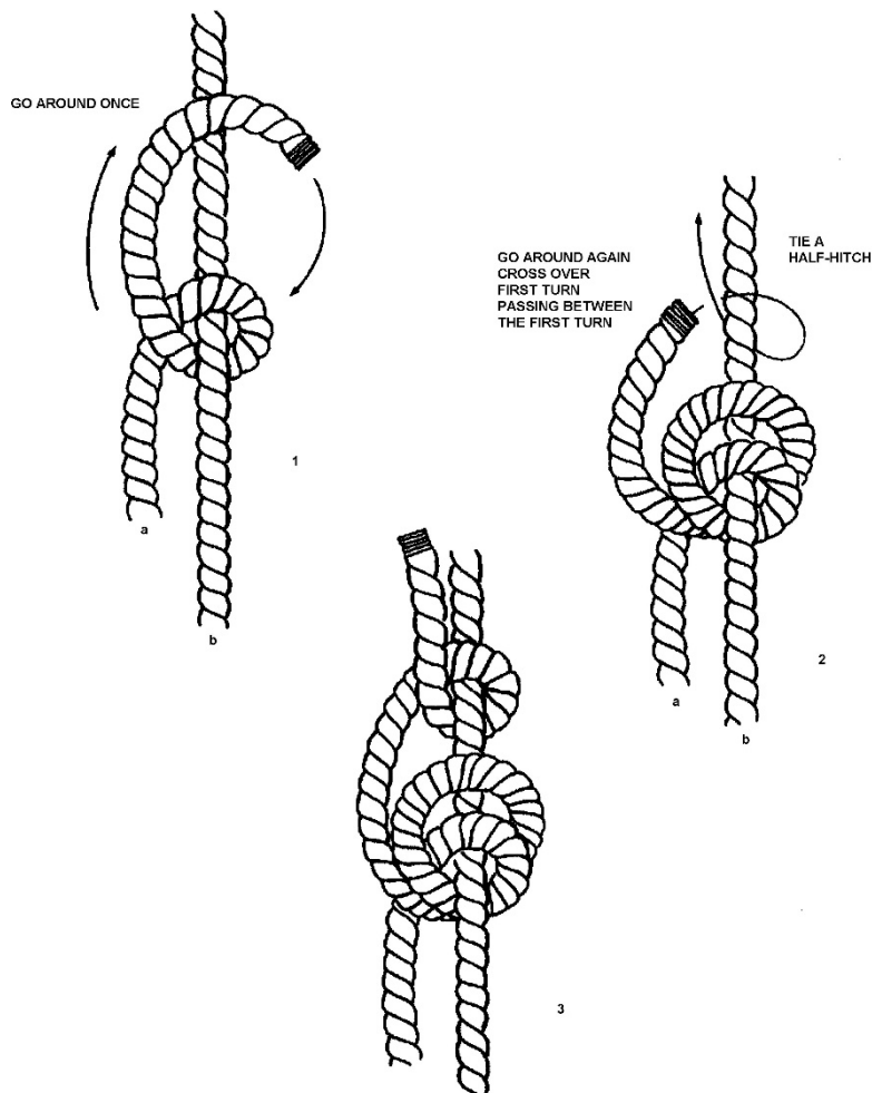
Figure 2-13 Rolling Hitch
