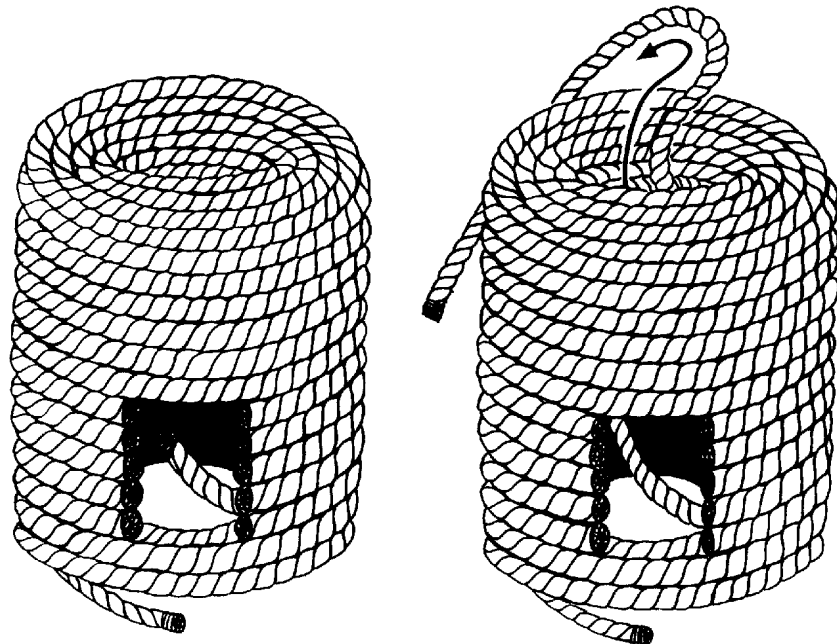
Figure 2-3 Opening a New Coil of Line
