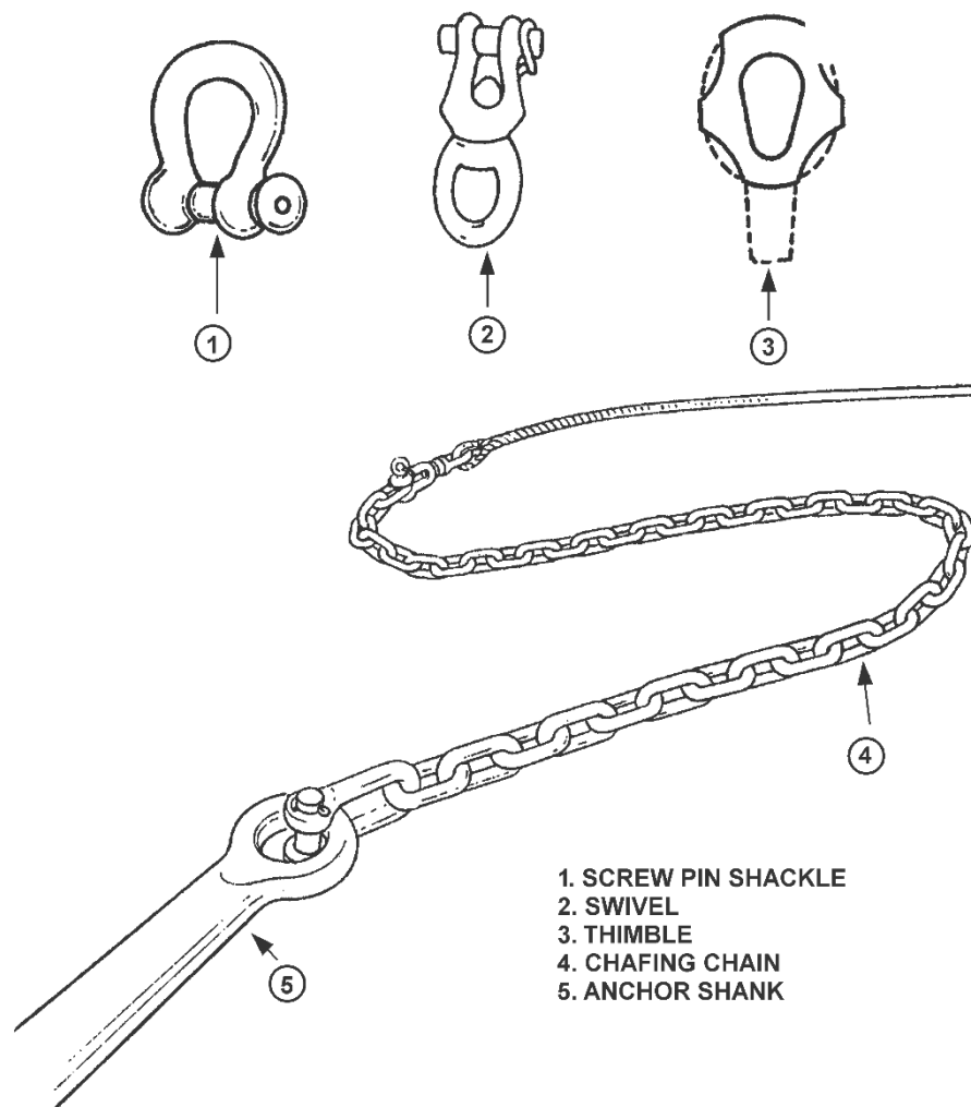
Figure 6-33 Anchor Fittings
