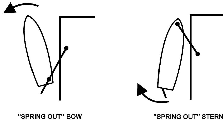
Figure 6-24 Basic Spring Line Maneuvers
