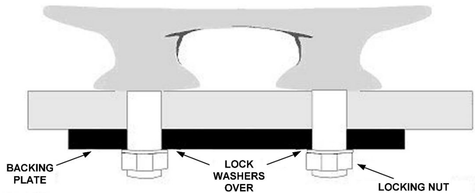
Figure 2-33 Backing Plate
