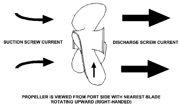
Figure 6-6 Screw Current
