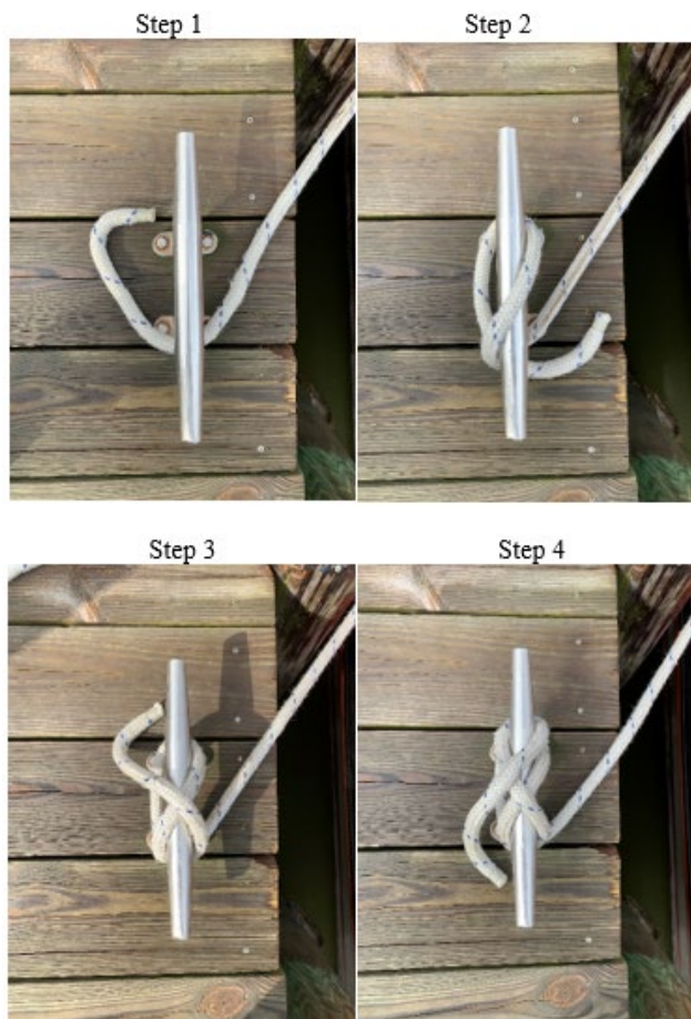
Figure 2-36 Securing a Line to a Cleat
