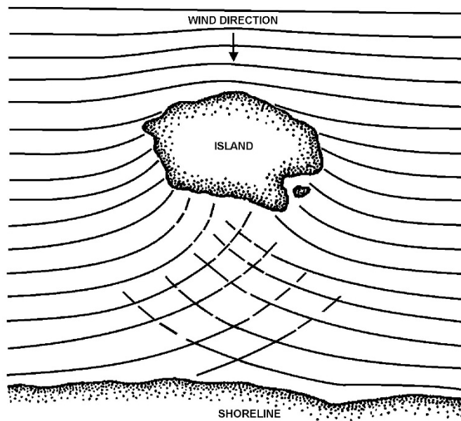
Figure 5-3 Wave Refraction
