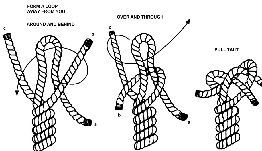
Figure 2-23 Crown Knot
