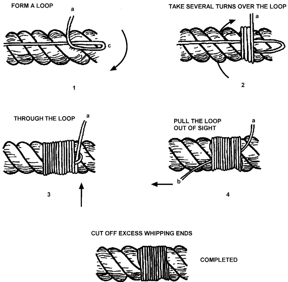
Figure 2-28 Temporary Whipping
