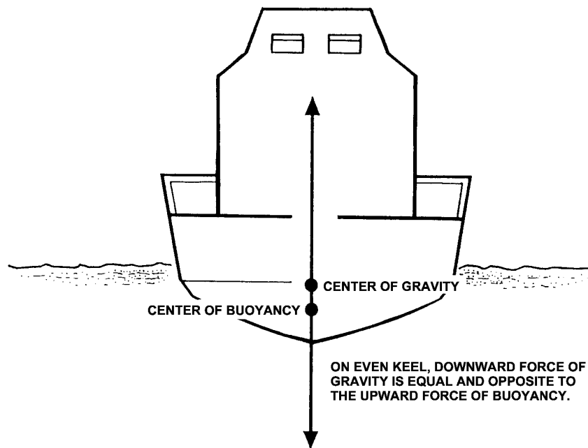
Figure 4-1 Stability in Equilibrium
