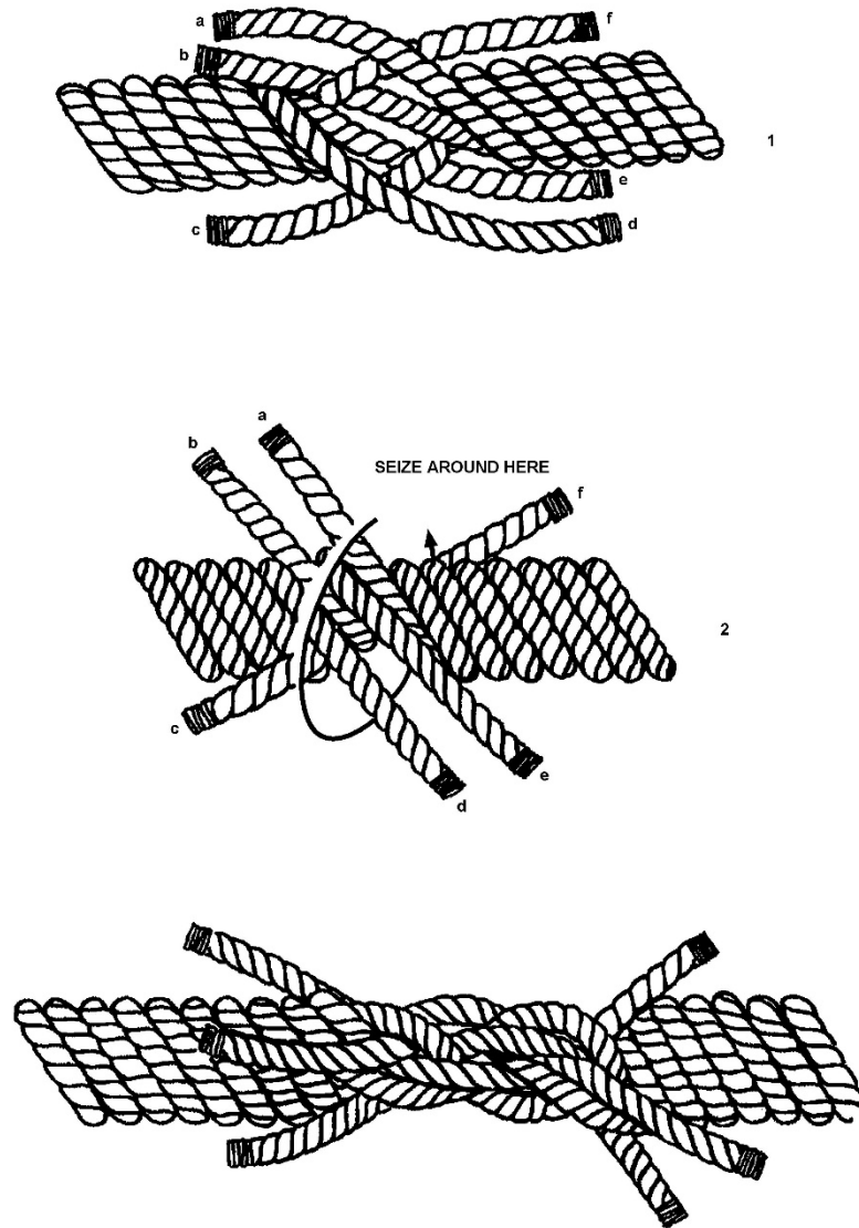
Figure 2-27 Short Splice
