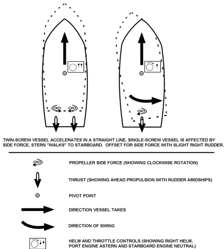
Figure 6-16 Accelerated Ahead
