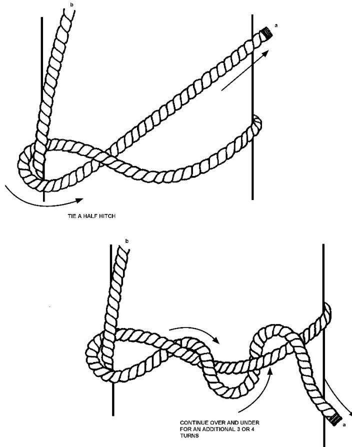
Figure 2-16 Timber Hitch
