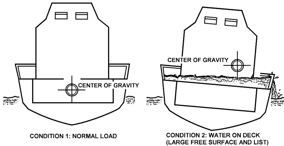
Figure 4-8 Effects of Water on Deck
