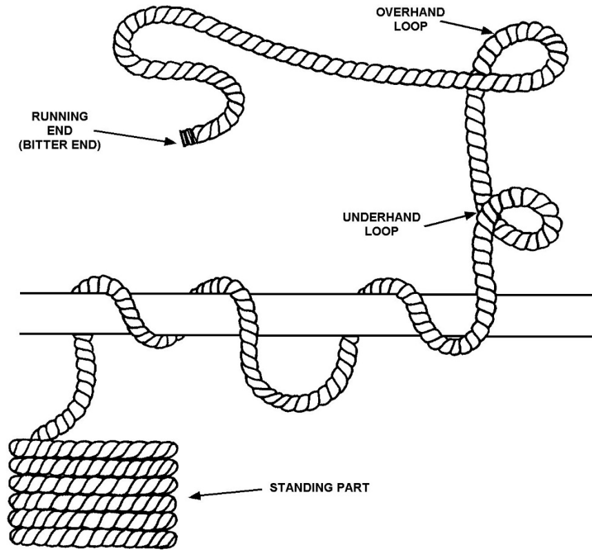
Figure 2-8 Basic Parts and Loops
