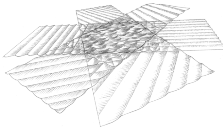
Figure 5-5 Wave Interference
