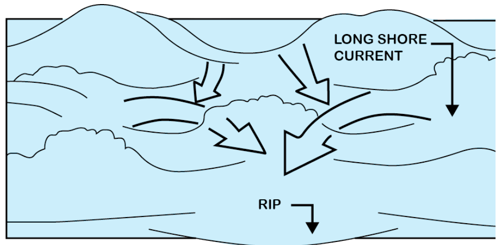
Figure 5-15 Rip Currents
