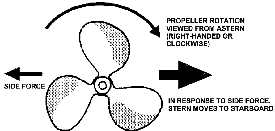
Figure 6-7 Side Force
