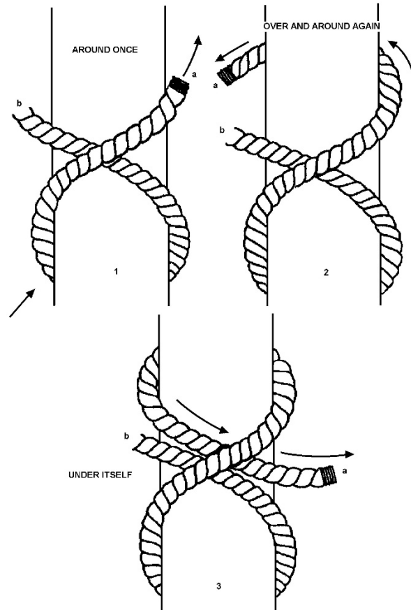
Figure 2-14 Clove Hitch
