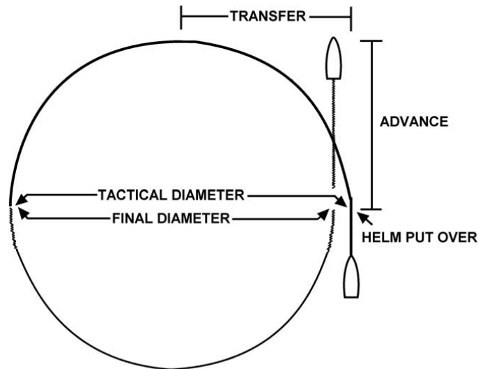
Figure 6-20 Turning Characteristics
