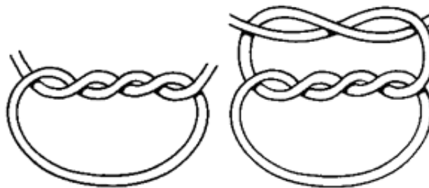
Figure 2-24 Surgeon’s Knot
