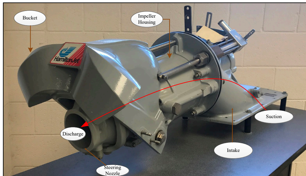
Figure 6-14 Waterjet
