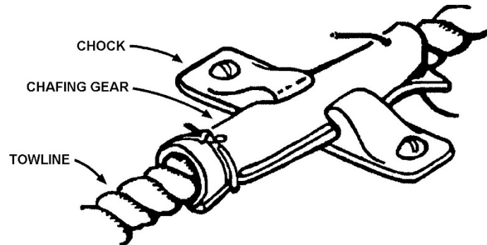
Figure 2-5 Chafing Gear
