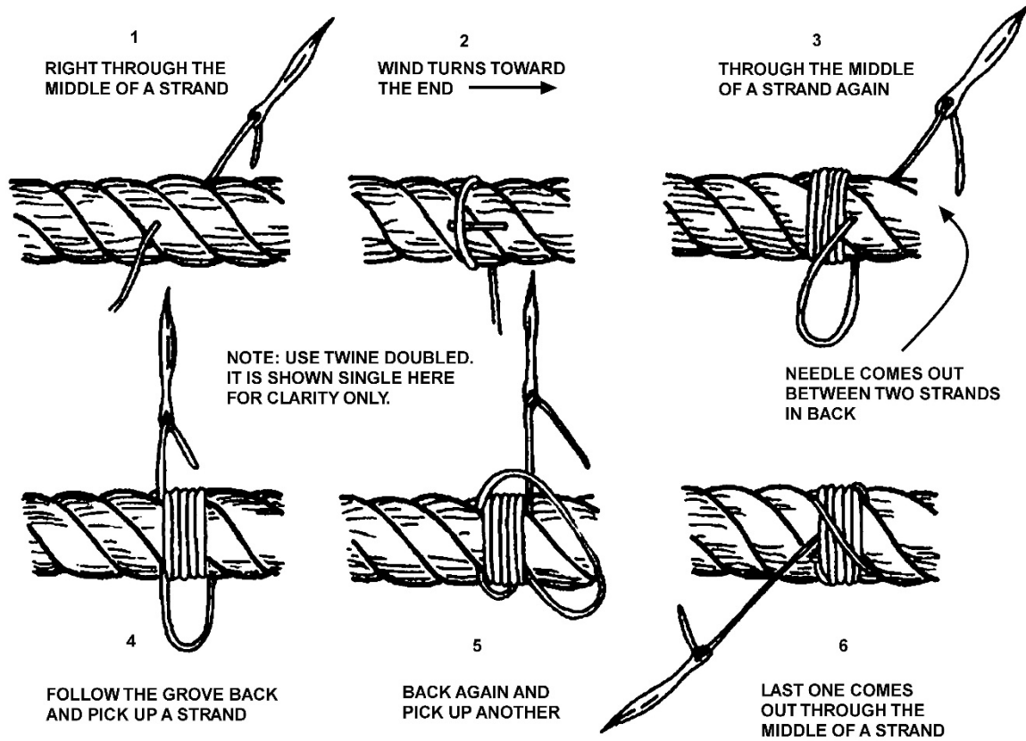
Figure 2-29 Permanent Whipping
